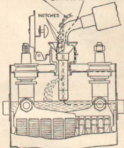
Diagram showing circuit of Electric Filler. Note that when solution reaches the correct level the end of filler nozzle just touches the solution, thereby completing the circuit and causing the bell to ring. The notches on the handle of filler give correct adjustment for different types of cells.
